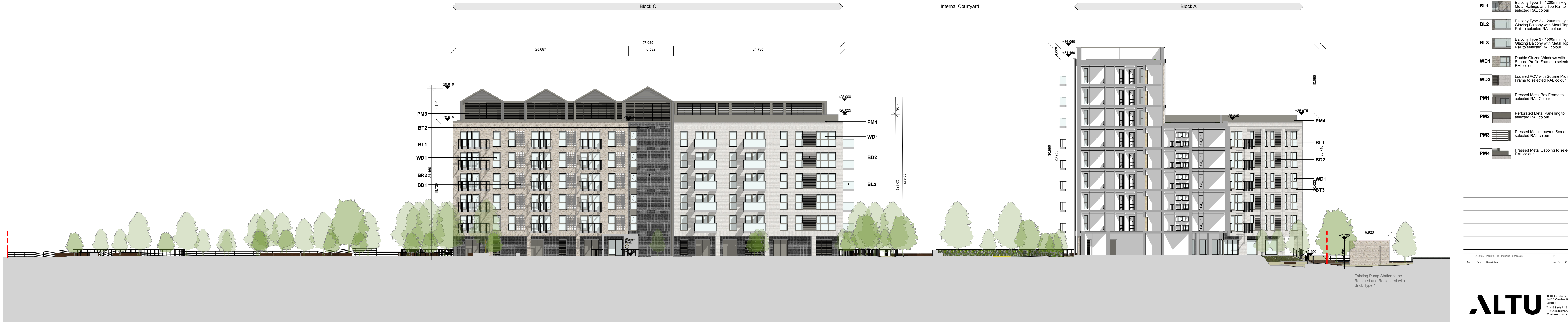
F-F Internal Courtyard Section Elevation - Block A SCALE: 1:200
