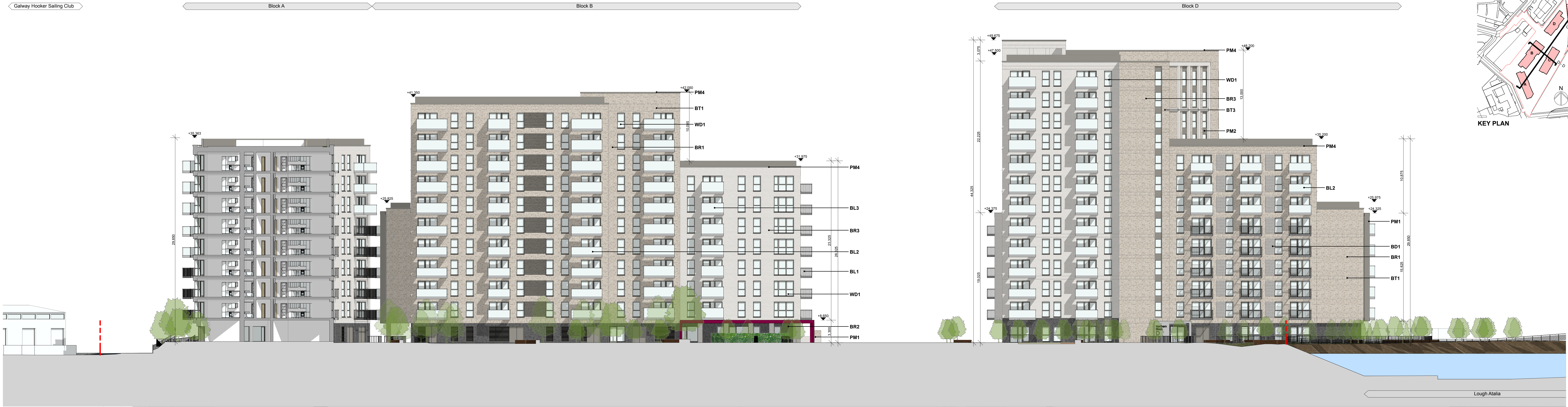
C-C Internal Courtyard Section Elevation - Block A & D SCALE:1:200
